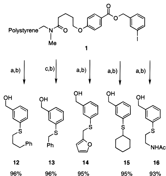
Scheme 3 a
