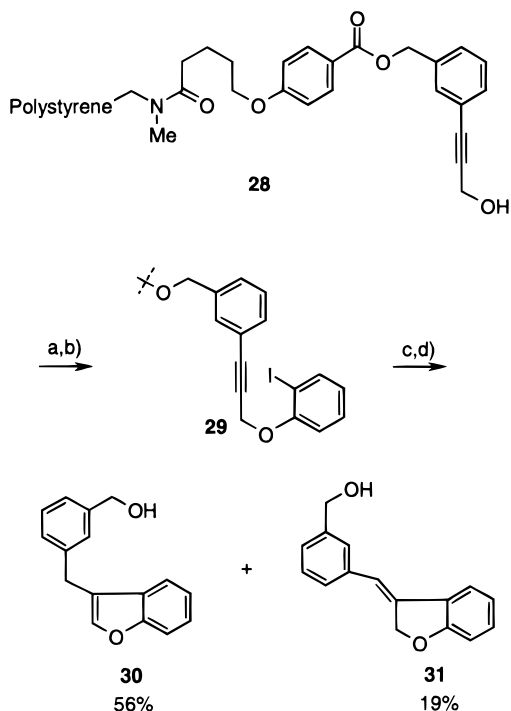
Scheme 7 a
