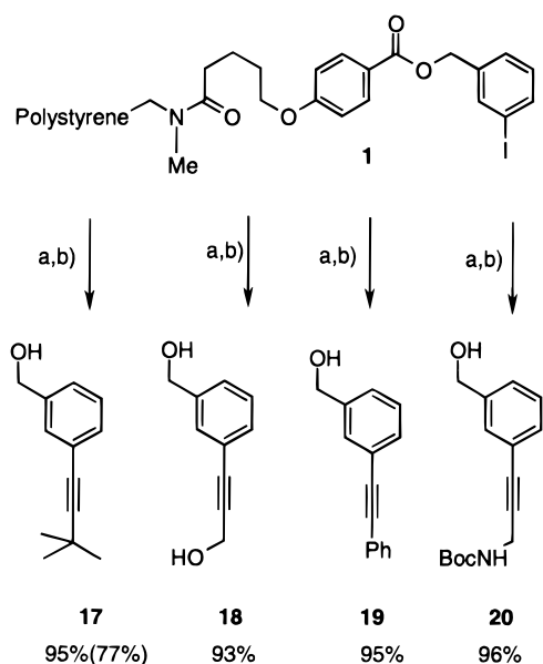
Scheme 4 a
