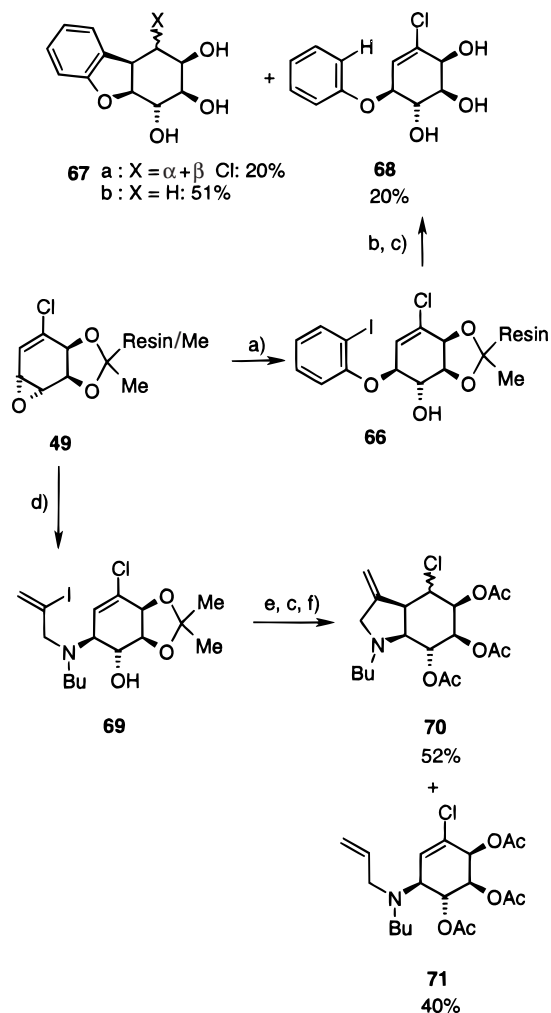
Scheme 15 a
